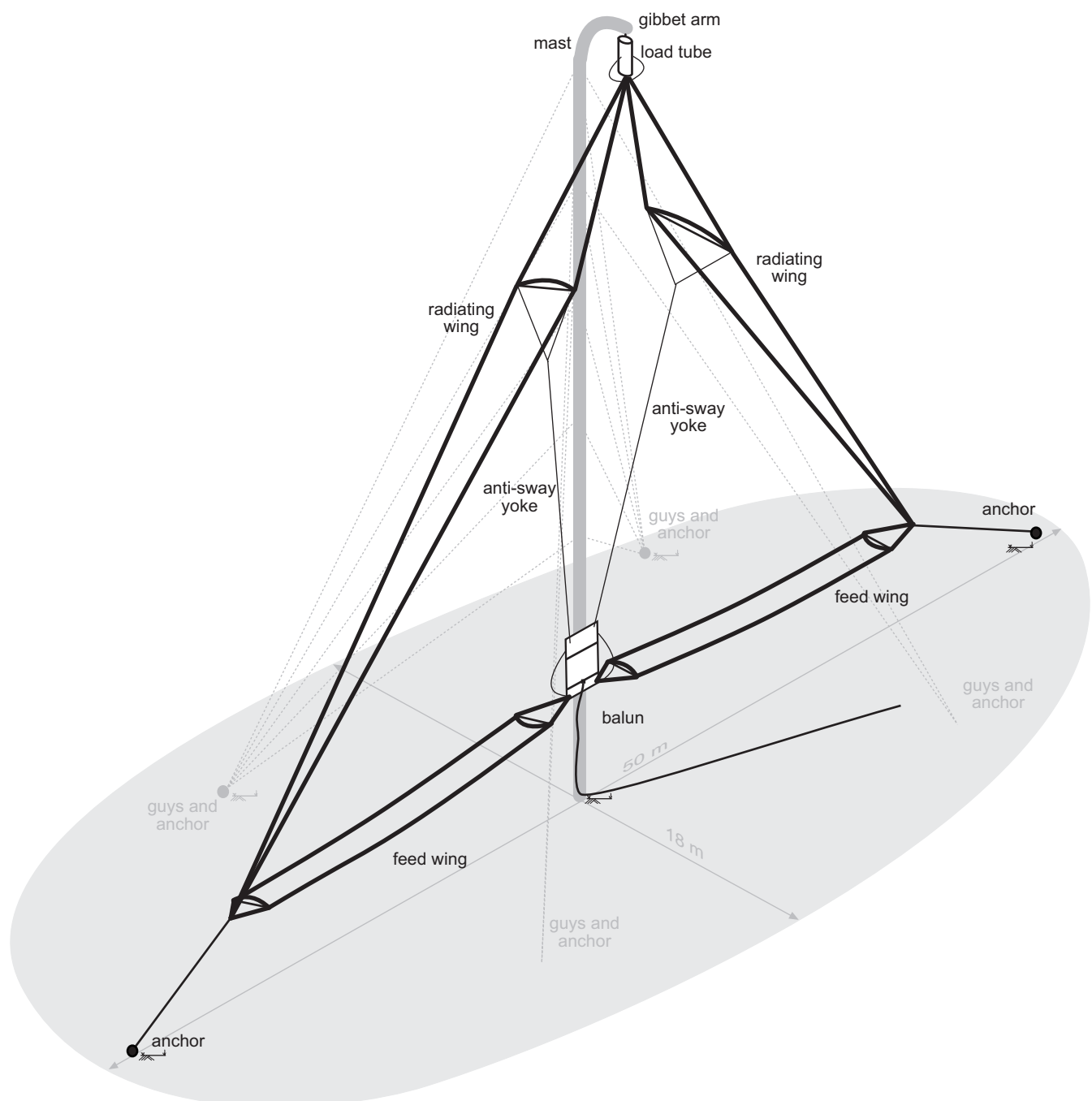
Figure 1: Delta antenna
